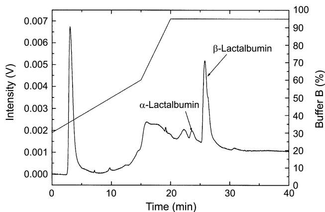
Fig. 3. Chromatogram of whey proteins after ultrafiltration (MWCO 30,000) from the fraction number #1 in Fig. 2 by RP-HPLC (Buffer A/Buffer B=70/30-40/60 vol%, gradient time of 15 min, Buffer A/Buffer B=40/60-5/95 vol%, gradient time of 20 min).
