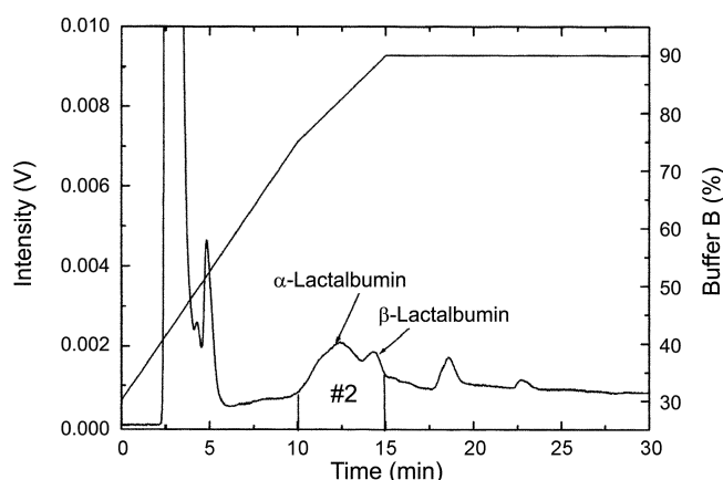
Fig. 4. Chromatogram of whey proteins after ultrafiltration (MWCO 30,000) by RP-HPLC (Buffer A/Buffer B=70/30-35/75 vol%, gradient time of 10 min, Buffer A/Buffer B=35/75-10/90 vol%, gradient time of 15 min).
